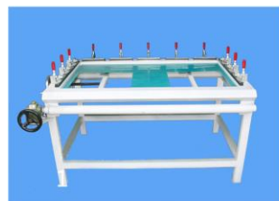
Screen Tighting
